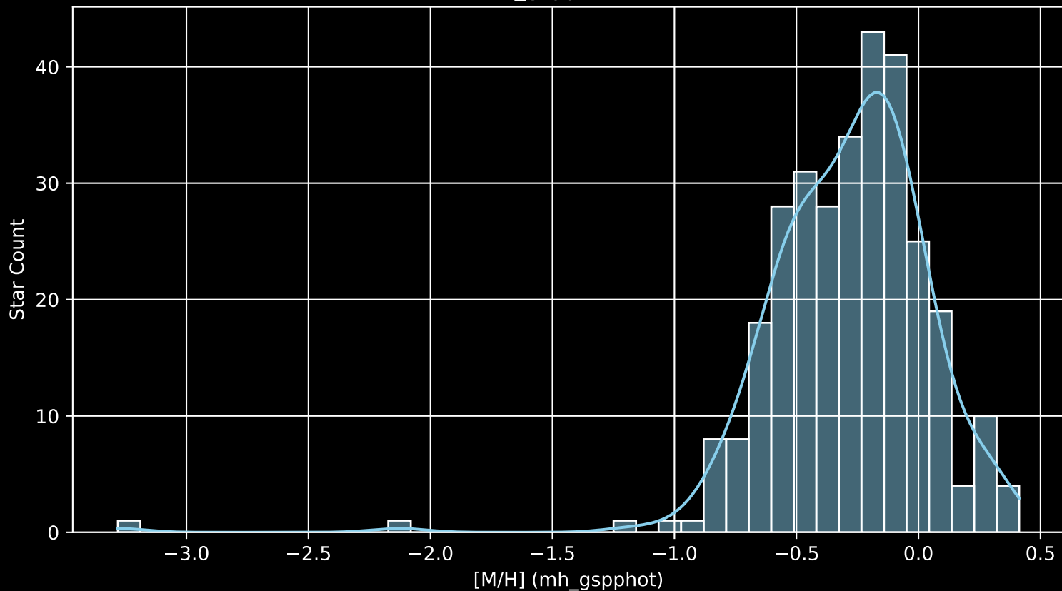
GALAH DR4 Field: [6962] [M/H] (mh_gspphot) (n= 306)
