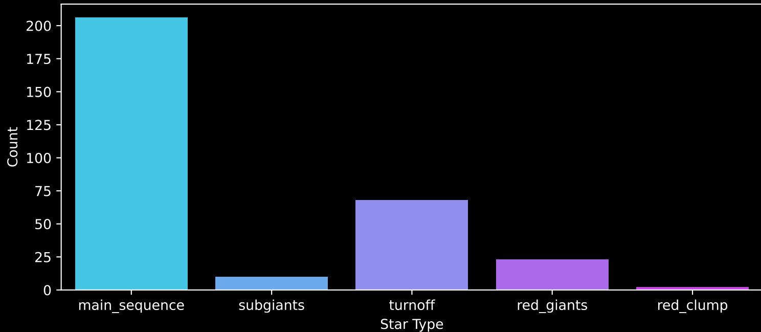
GALAH DR4 Field: [6962] Count plot of Star Type
