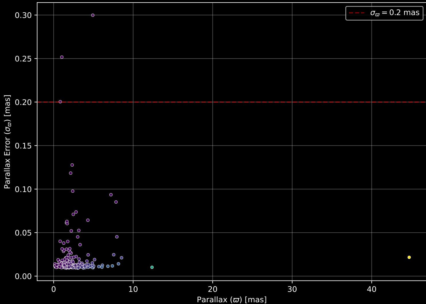
GALAH DR4 Field: [6962] Parallax Quality (n= 309)
