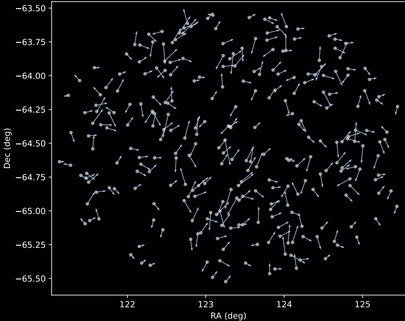
GALAH DR4 Cluster 1 Proper Motion Vectors (n=273)
