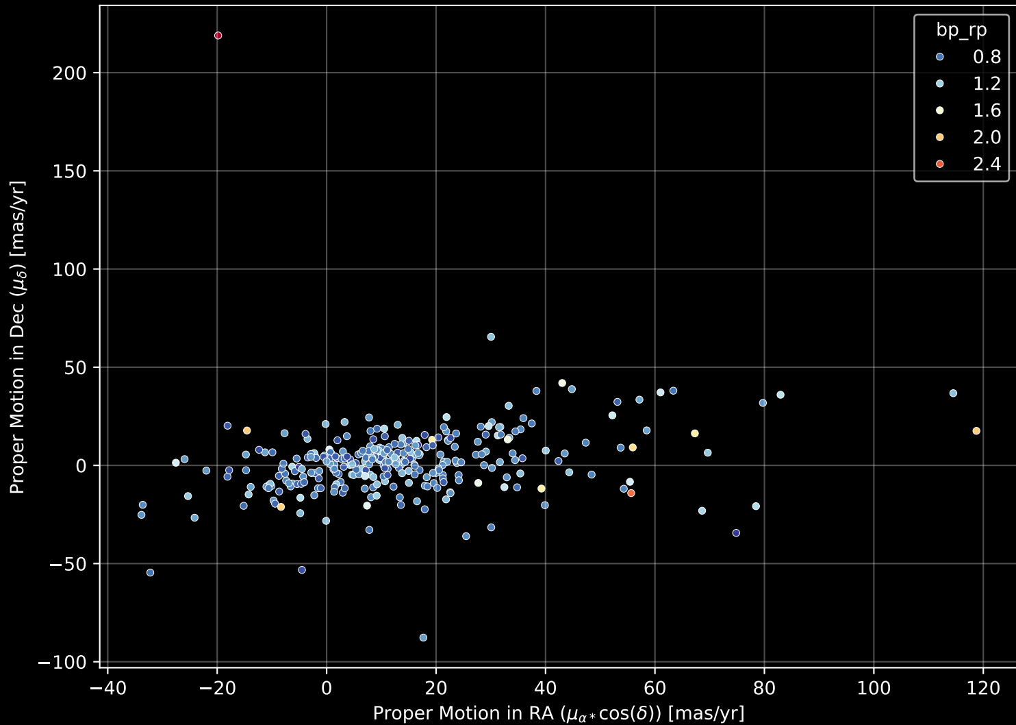
GALAH DR4 Field: [6962] Proper Motion Diagram (n= 309)
