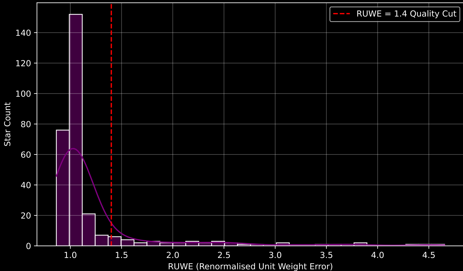
GALAH DR4 Field [6962] RUWE Distribution (n= 297)
